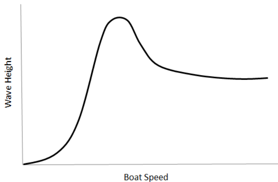
Figure 4. Wave height as a function of speed in planing hull vessels. Adapted from Maynard 2001.
