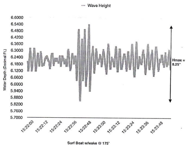
Graphs 3-8 - Surface wave measurements for wake boats at varying distances from shore.
