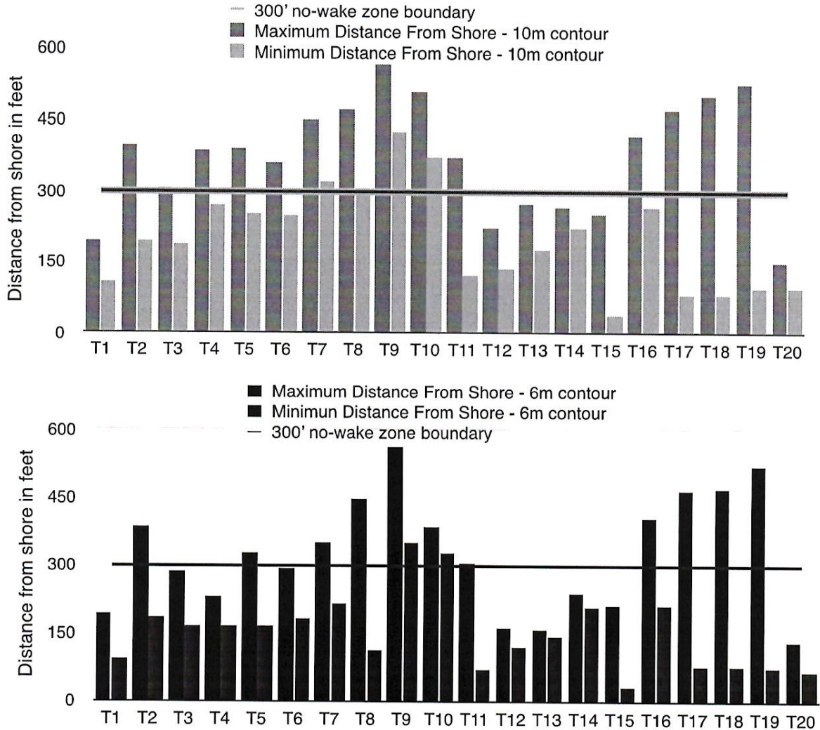
Graph 1-2 - 10m and 6m depth contour max. and min. distance from shore.
