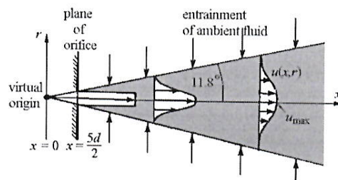
Fig. 1 - Establishment of slipstreams for turbulent, non-buoyant jets. 3
