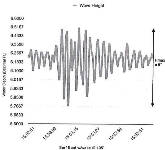
Graphs 3-8 - Surface wave measurements for wake boats at varying distances from shore.
