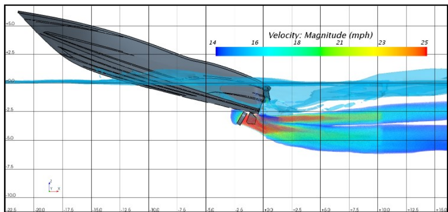
Figure 33. Propeller wash velocity (25 mph = 36.7 ft/sec).
