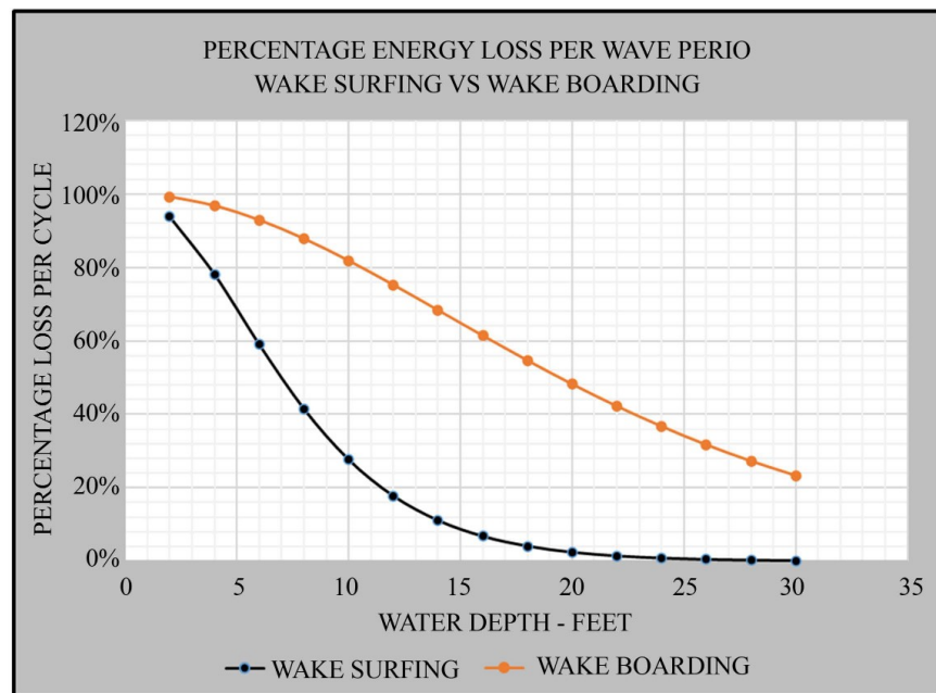
Figure 31. Percentage energy loss per wave period.
