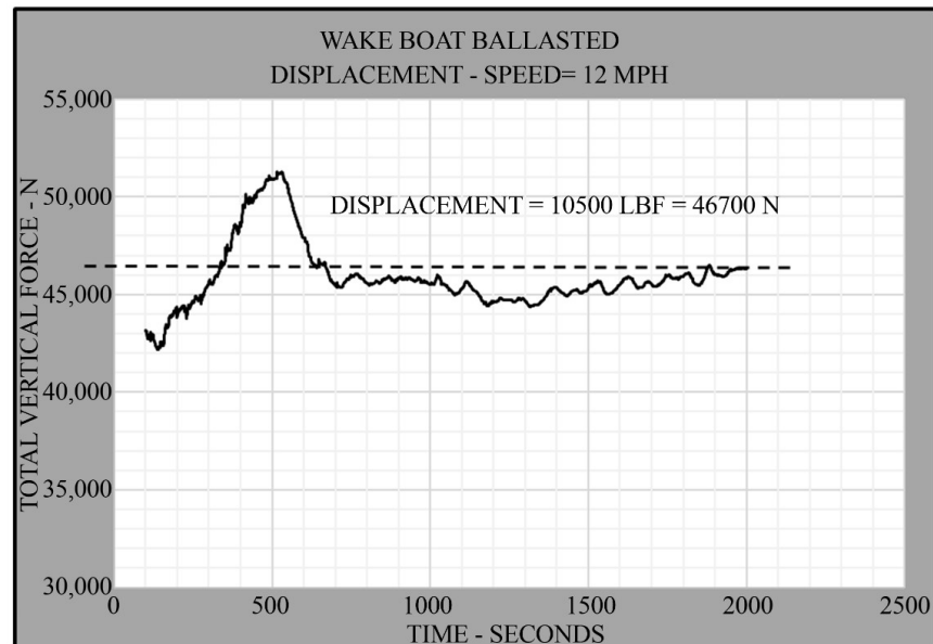
Figure 13. Convergence of vertical force.
