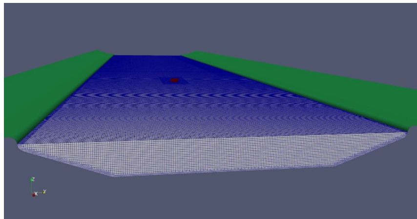
Figure 9. Channel model showing the water mesh.
