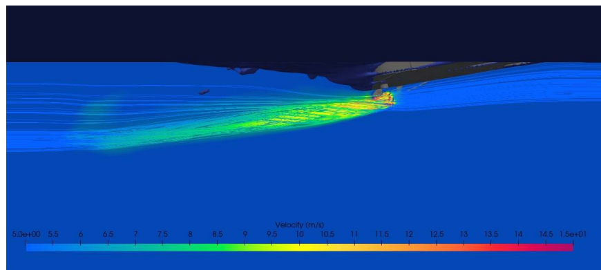
Figure 34. Propeller streamlines showing vertical mixing.
