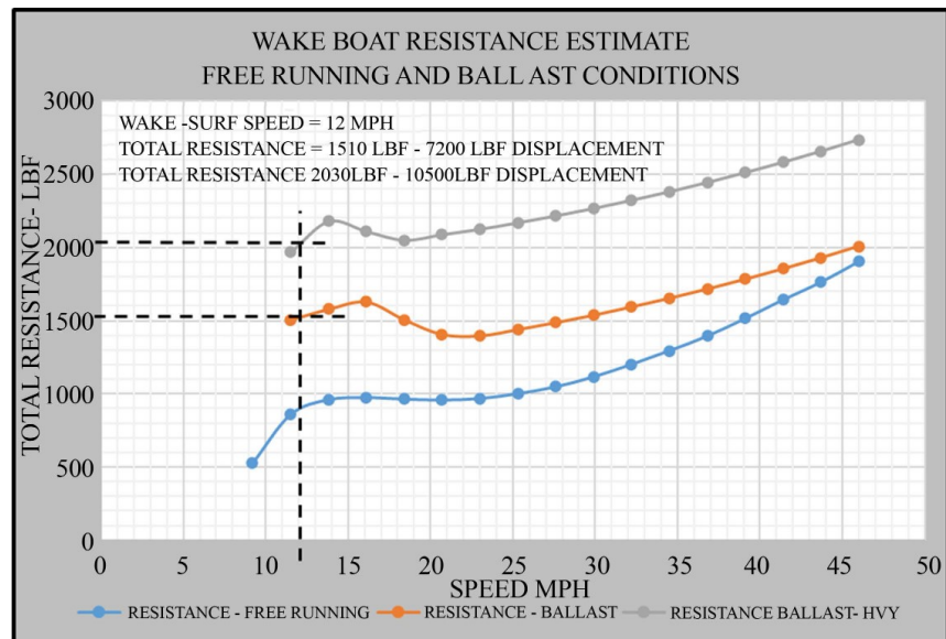
Figure 3. Wake boat resistance estimate.
